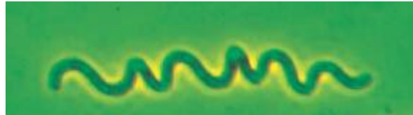
Rhodospirillum rubrum
